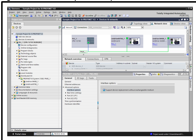
Figure 9-6 PLC device replacement option
